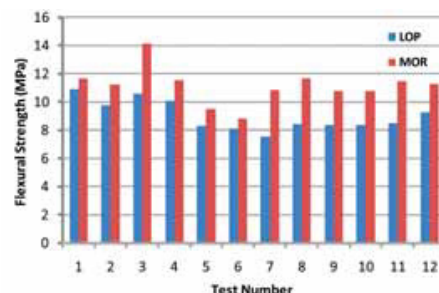
Figure 2: Typical flexural strengths (non-polymer) from daily QC tests
